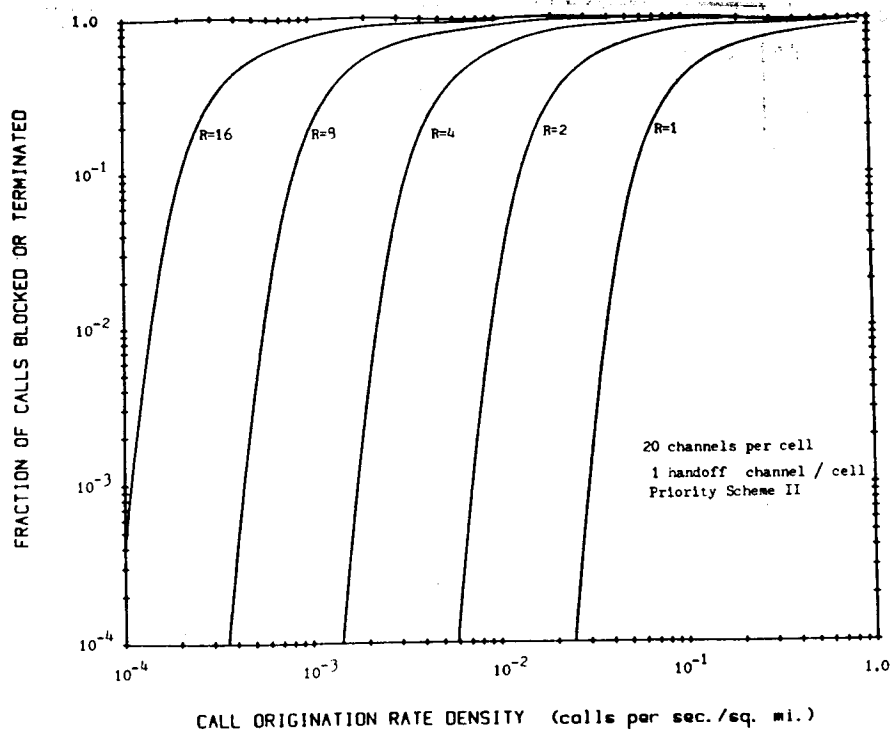
Fig. 9. Fraction of new calls uncompleted (Priority Scheme II, 20 channels/cell, 1 handoff channel/cell).
