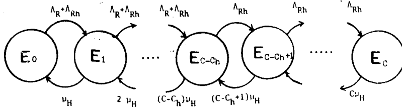
Fig. 1. State-transition diagram for Priority Scheme I.
